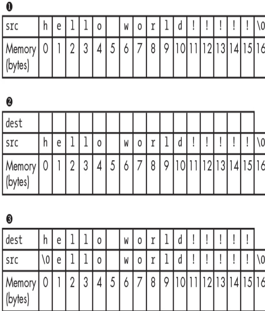
Figure 13-1: How memory overflows from dest to src
